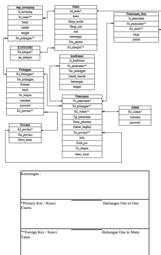
Gambar 25 Relationship Between Tables
