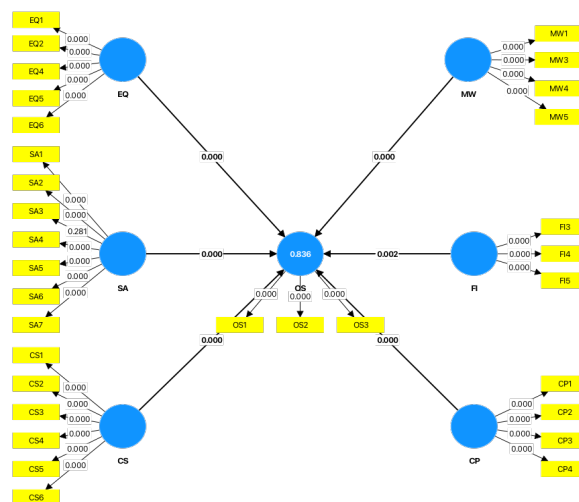
Figure 1. Path Algorithm Result from SmartPLS
